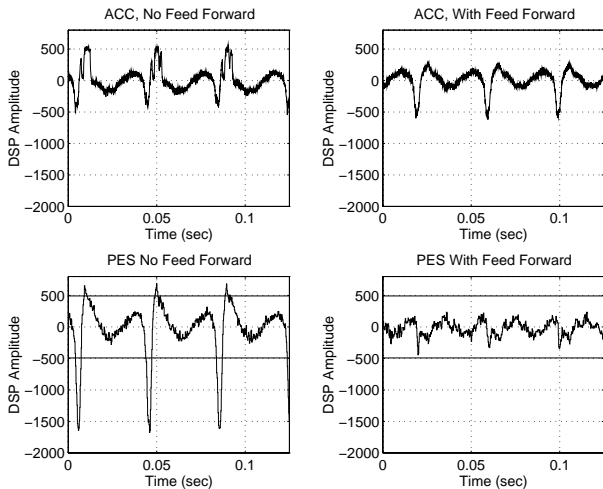
Fig. 13. Adaptation during intermittent 3 mS shock pulses. Note that even though the magnitude of the pulses does not change, their effect on the system does. The thresholding routine keeps the parameters from drifting in between shock pulses.
