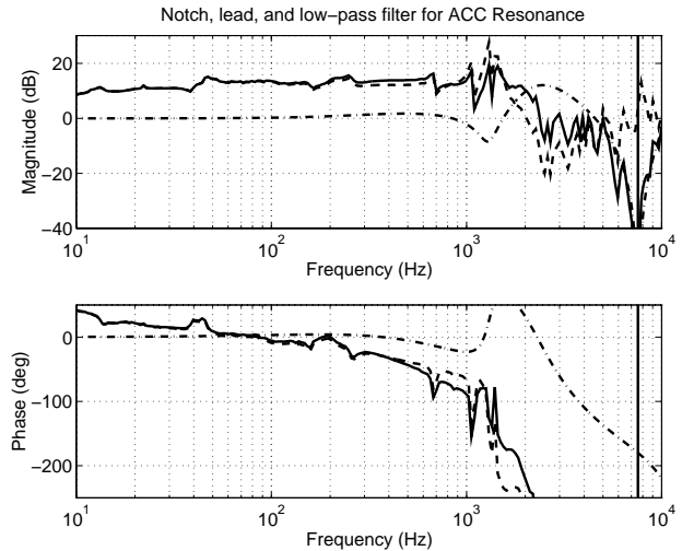
Fig. 6. Frequency response of accelerometer plus lead, notch and low pass filter. The accelerometer signal is sampled at 4 times the nominal rate. The dashed line represents the accelerometer frequency response, the dashed-dotted line is the frequency response of the filter, and the combined response is shown by the solid line. The vertical solid line is at the Nyquist frequency of 7434 Hz.
