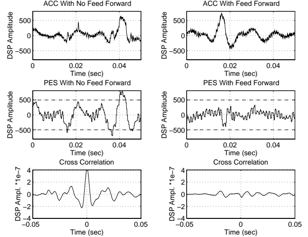
Fig. 12. Comparison of signal correlations. The top two plots have the accelerometer signals, the center two plots have the PES signals, and the bottom two have the cross correlation between the two. On the left hand side it is clear that with no feedforward ACC and PES are highly correlated. On the right hand side, it is clear that once the algorithm has adjusted the gain, the correlation is considerably reduced.
