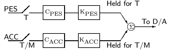
Fig. 9. Compensator structure. C_{(\cdot)} is the compensator filter, K_{(\cdot)} is the gain.
