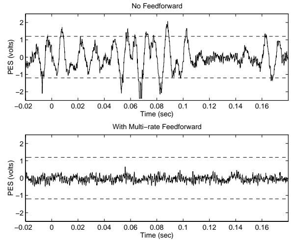
Fig. 8. Multi-rate feedforward of in drive rotational accelerometer signal (ACC). ACC is sampled at 4X the nominal sample rate. This is with a tuned filter gain.
