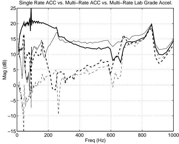
Fig. 7. Comparison of frequency response functions from disturbance to PES. In this plot, the farther down the plot, the more suppressed the disturbances are. The thick solid line is without feedforward. The thin solid line is with the on drive accelerometer (ACC) being fed forward with single rate sampling. The thick dashed line is with ACC being fed forward with 4X multi-rate sampling. The thin dashed line is with the signal from a laboratory grade accelerometer being fed forward with 4X multi-rate sampling. Note that with the proper filtering and a high enough sample rate, the in drive accelerometer can nearly match the laboratory grade accelerometer over a large frequency range in its usefulness for disturbance rejection.
