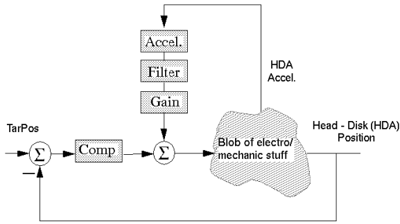
Fig. 3. Block Diagram of Feedforward Cancellation
