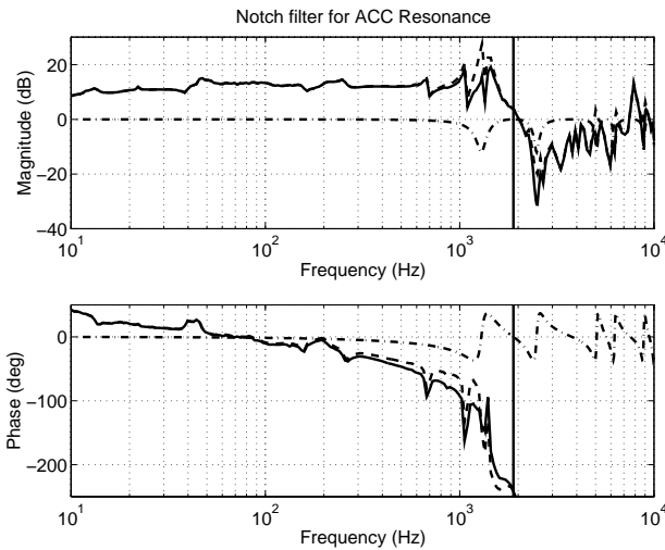
Fig. 4. Frequency response of accelerometer and notch filter. The accelerometer signal is sampled at the nominal rate. The dashed line represents the accelerometer frequency response, the dashed-dotted line is the frequency response of the filter, and the combined response is shown by the solid line. The vertical solid line is at the Nyquist frequency of 1858.5 Hz.
