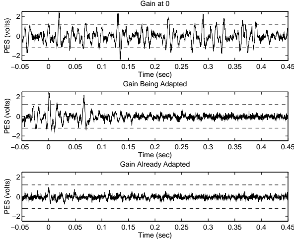
Fig. 11. Adaptation of accelerometer filter gain. Note the rapid decrease in the magnitude of the position error. The disturbance is random rotary vibration between 50 and 150 Hz with a level of 57.7 \text{ rad/s}^2 rms.
